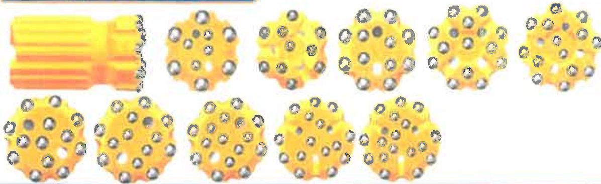
T45 Button bits, retract skirt
